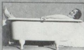
Partial Eclipse
